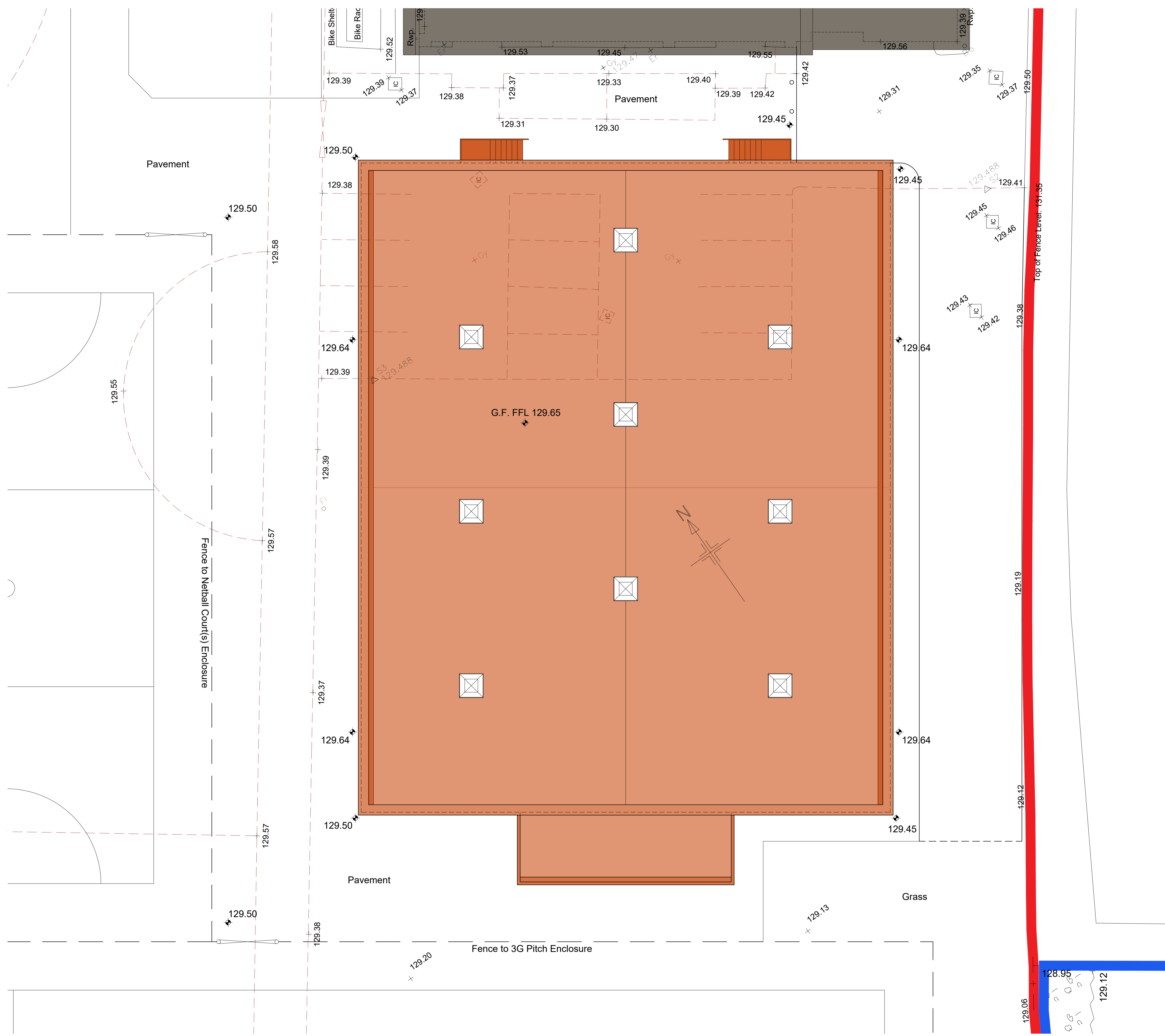
PROPOSED ASSEMBLY HALL - BLOCK PLAN Scale 1:100 @ A1
